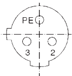
Female connector 2-pos.+PE
