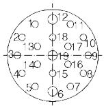
Female connector
